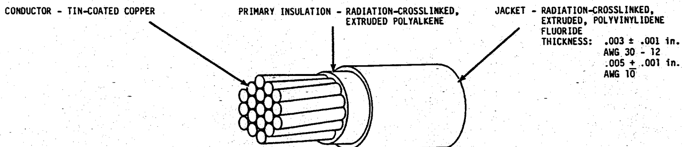
Figure 1 - Construction of Finished Wire
